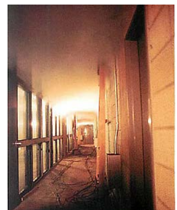
Smoke movement test at corridor
