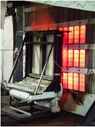
Fire Tests on building materials/products used at interior and/or exterior of buildings
