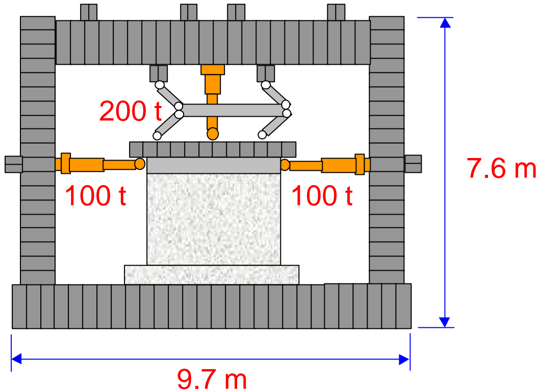
Reaction frame to be installed at UTCB
